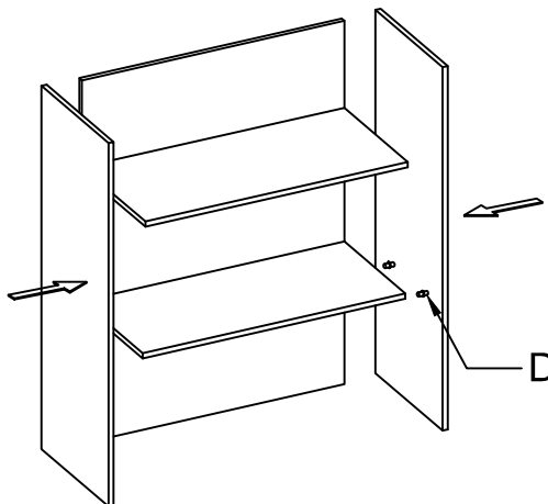
Middle partition plate :770x365x15=1
