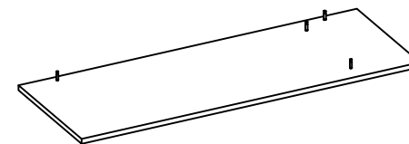
Right side plate :1050x380x15=1
